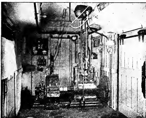
Fig. 149. ELECTRIC LIGHT PLANT. CHICAGO, MILWAUKEE & ST. PAUL RAILWAY. (Placed in the end of Baggage Cars.)
